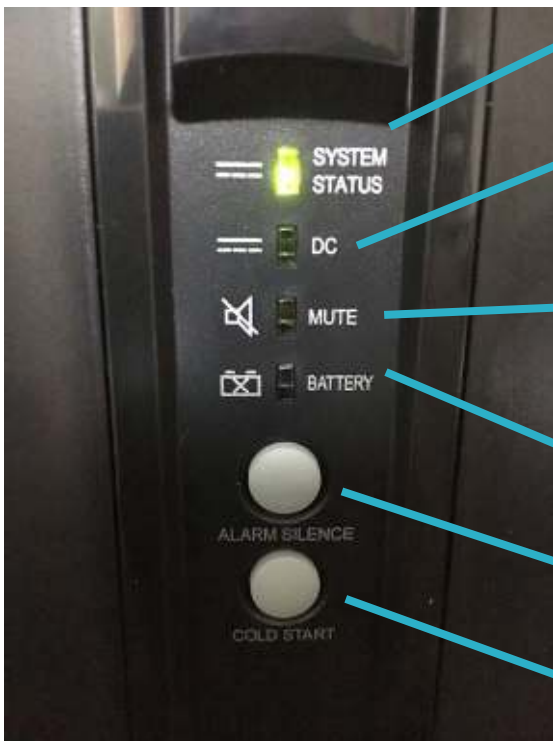
Front Panel of Battery Backup Unit.*
